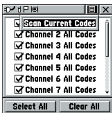
Scanlist Options.
