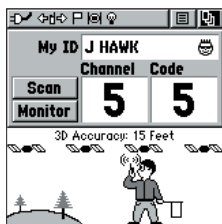
Radio Page
